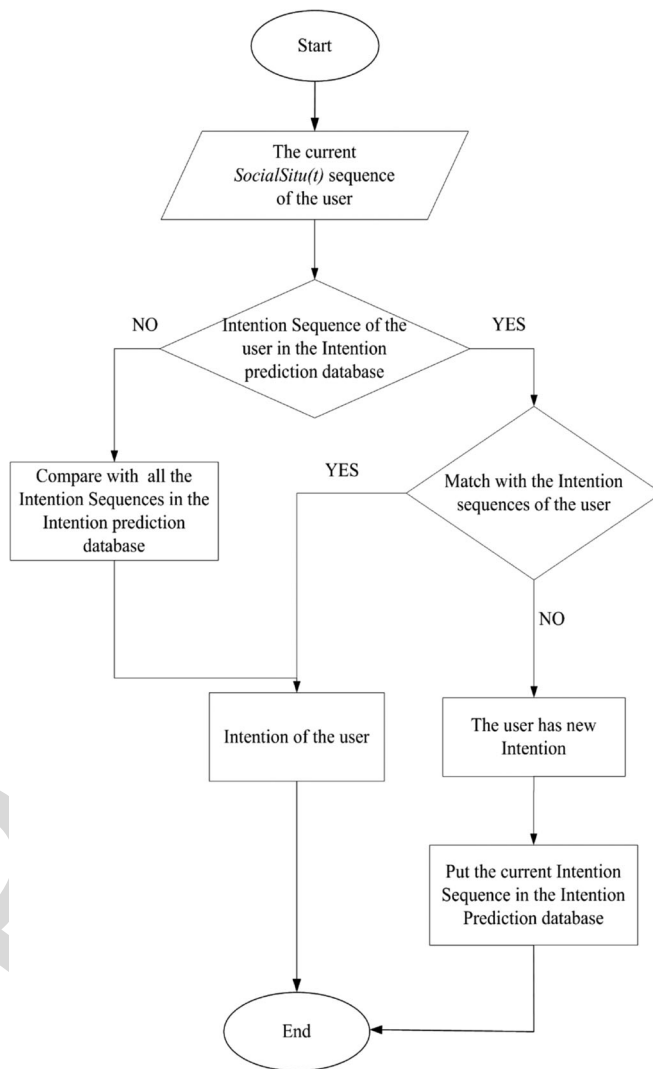
Fig. 2. Intention prediction flowchart of the user.
