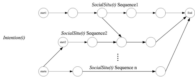
Fig. 1. Intention sequence.
