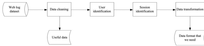
Fig. 4. Data preprocessing for intention serialization algorithm.
