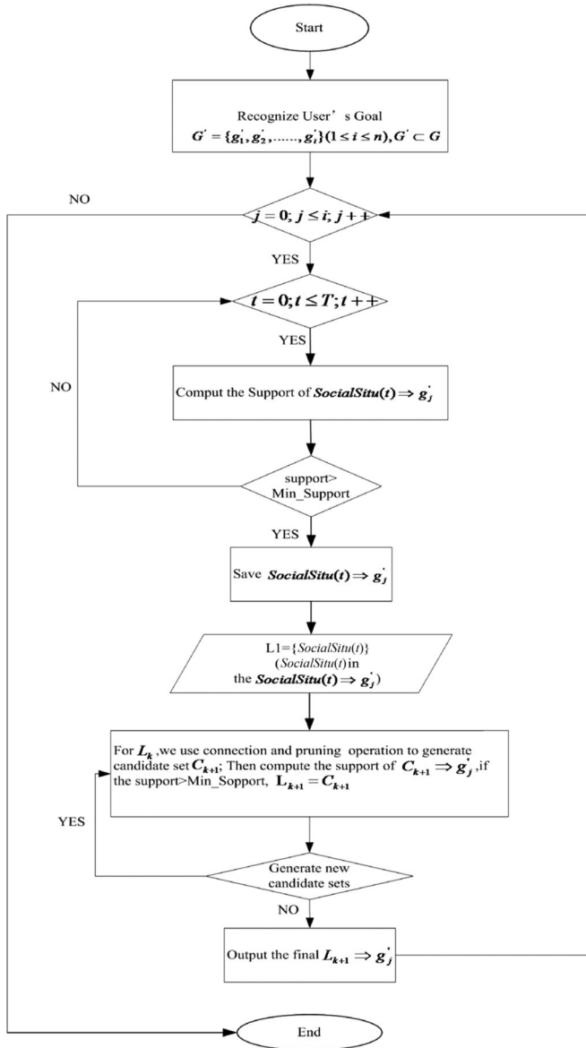
Fig. 3. Flowchart of situational aware intention serialization algorithm.
